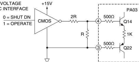
FIGURE 1c. THERMALLY ACTIVATED SHUTDOWN
