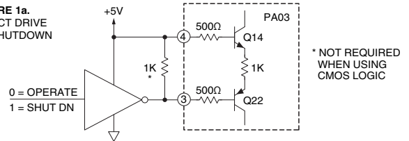
FIGURE 1b. HIGH VOLTAGE LOGIC INTERFACE
